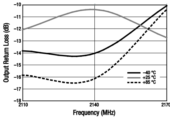
Figure 7. Output Return Loss vs Frequency Over Temperature With Maximum Attenuation
