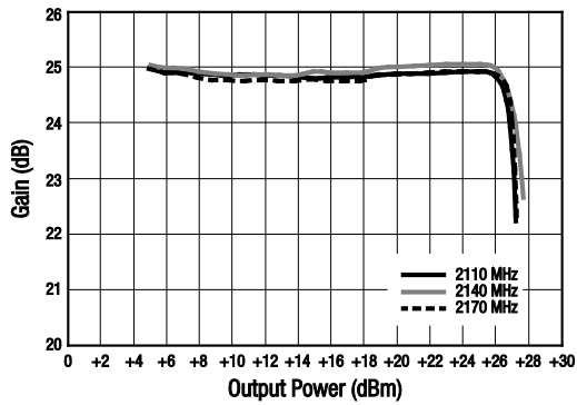
Figure 9. Gain vs Output Power Over Frequency
