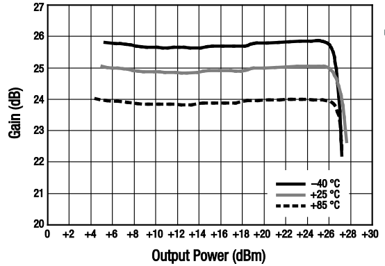
Figure 10. Gain vs Output Power Over Temperature
