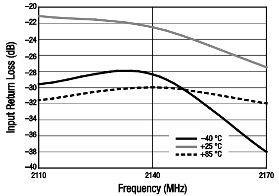
Figure 4. Input Return Loss vs Frequency Over Temperature With Minimum Attenuation
