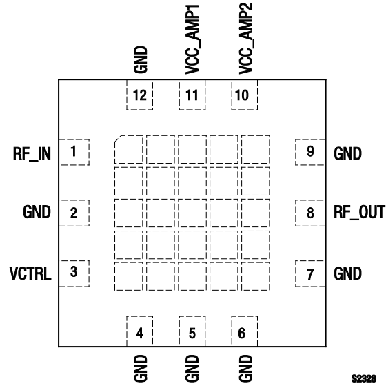
Figure 2. SKY65187-11 Pinout – 12-Pin MCM (Top View)
