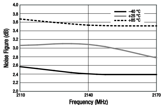
Figure 19. Noise Figure vs Frequency Over Temperature
