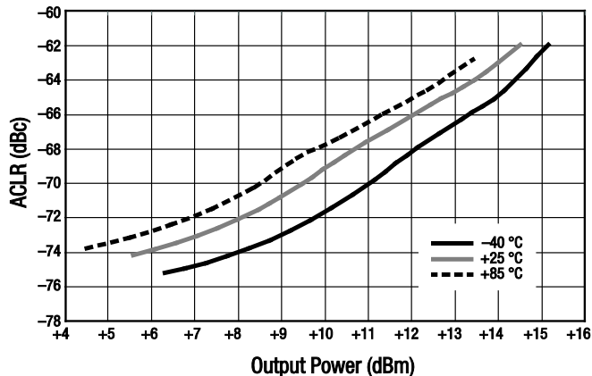
Figure 17. ACLR vs Output Power Over Temperature (WCDMA Test Model 1 With 64 DPCH)
