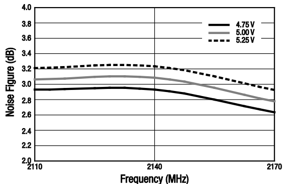
Figure 18. Noise Figure vs Frequency Over Voltage
