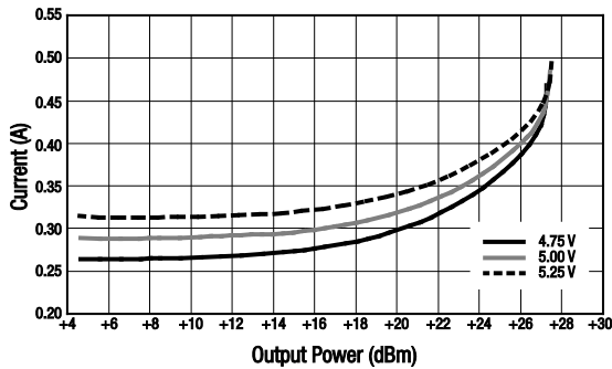
Figure 11. Current vs Output Power Over Voltage
