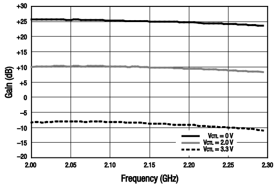
Figure 8. Gain vs Frequency Over Control Voltage
