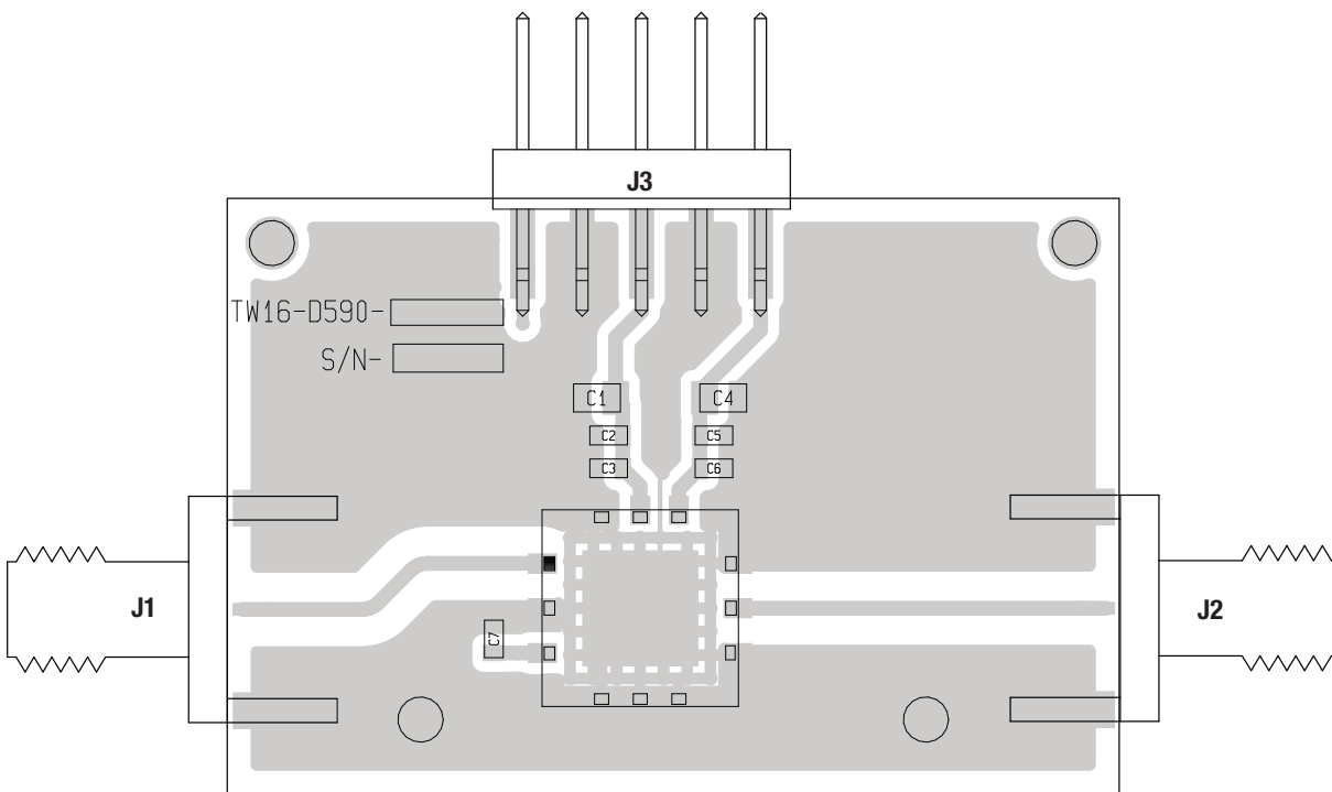
Figure 21. SKY65187-11 Evaluation Board Assembly Drawing
