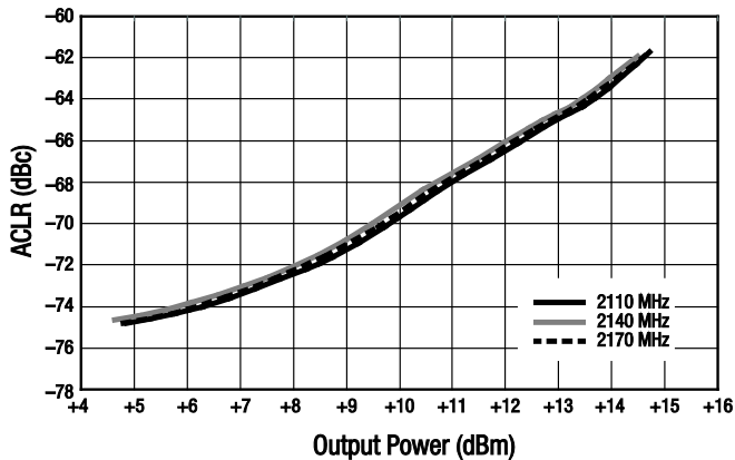
Figure 16. ACLR vs Output Power Over Frequency (WCDMA Test Model 1 With 64 DPCH)
