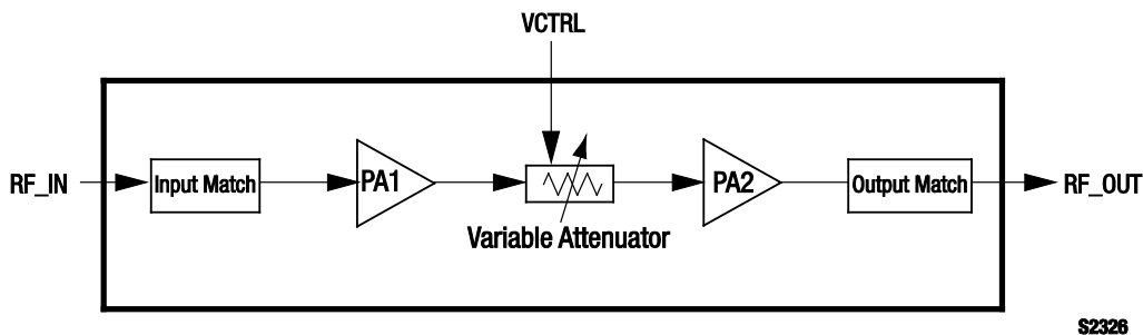
Figure 1. SKY65187-11 Block Diagram
