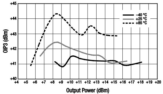
Figure 14. OIP3 vs Output Power Over Temperature
