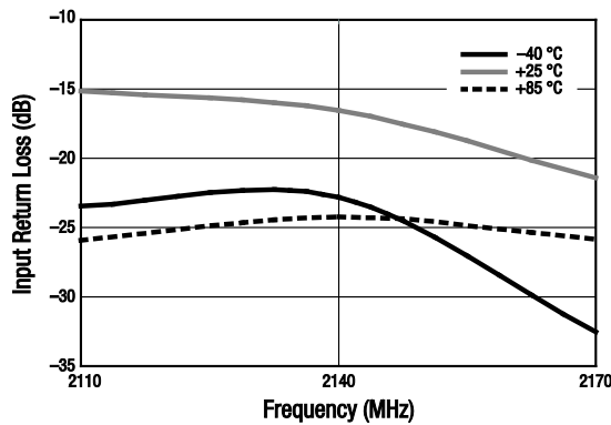
Figure 5. Input Return Loss vs Frequency Over Temperature With Maximum Attenuation
