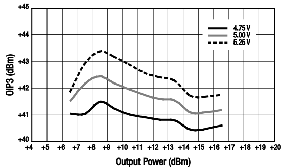
Figure 15. OIP3 vs Output Power Over Voltage
