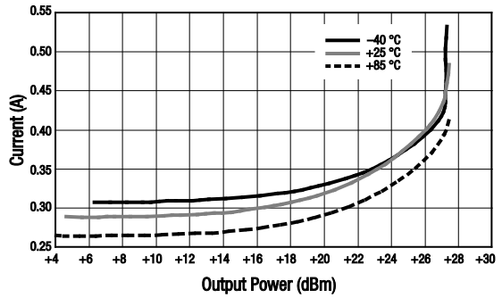
Figure 12. Current vs Output Power Over Temperature
