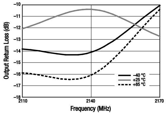
Figure 6. Output Return Loss vs Frequency Over Temperature With Minimum Attenuation
