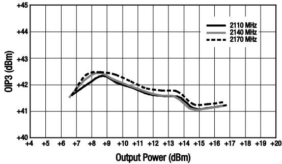
Figure 13. OIP3 vs Output Power Over Frequency
