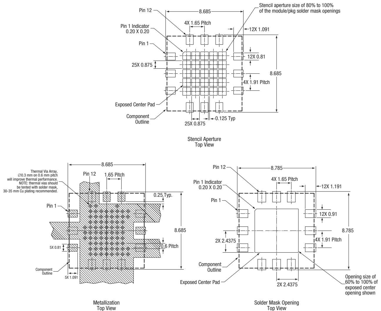
Figure 24. SKY65187-11 PCB Layout Footprint
